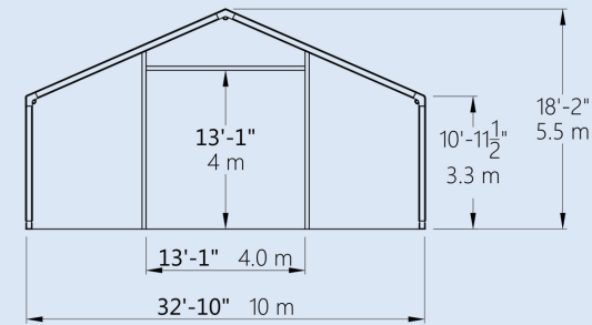
EXTERIOR DIMENSIONS
