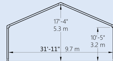
INTERIOR DIMENSIONS
